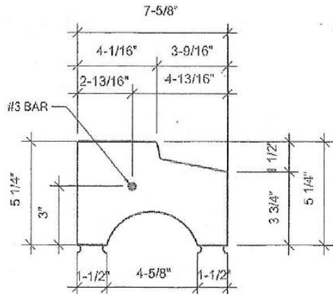
Deep Face Flush Utility / Thick Finish Flush Product Code: DFFU
