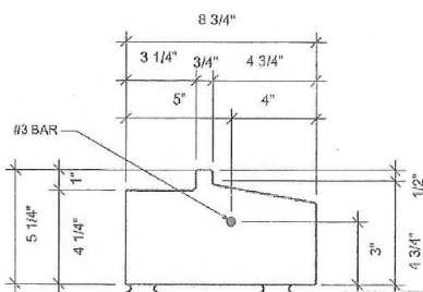
Deep Face / Thick Tile Sill Product Code: DF
