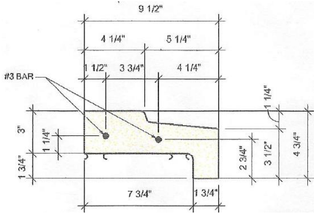
Wind Resistant Face / Wind Tile Sill Product Code: F
