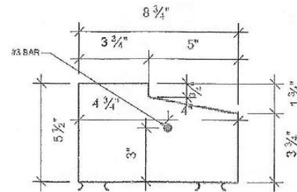
Deep Face Utility / Thick Finish Sill Product Code: DFU
