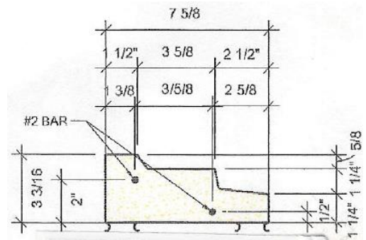
3-Step Storm Stop / 3-Step Product Code: 3S
