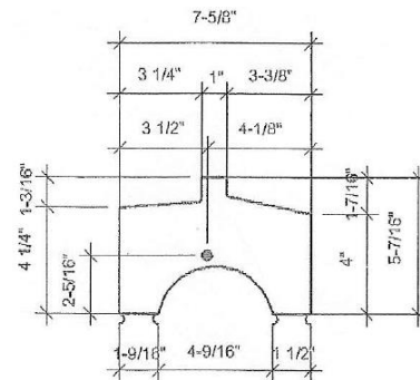
Deep Face Flush / Thick Flush Sill Product Code: DFF
