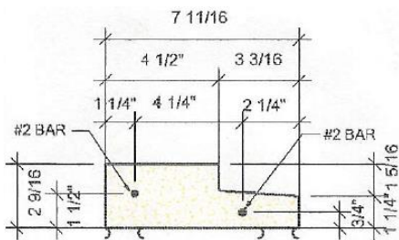
Wind Resistant / Wind Sill Product Code: WR
